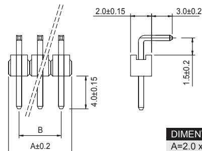
SINGLE ROW-RIGHT ANGLE
