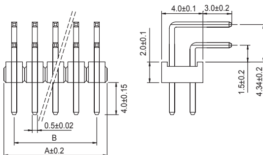
DOUBLE ROWS-RIGHT ANGLE
