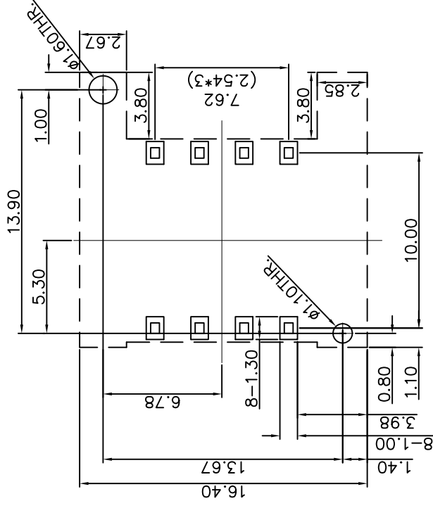
REFERENCE PC BOARD LAYOUT
